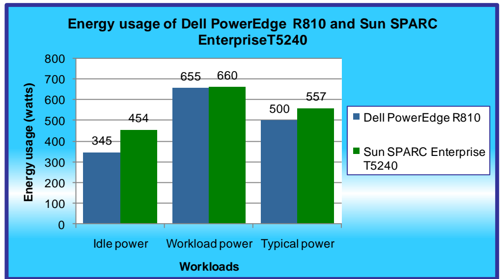
Figure 5: Server energy usage estimates based on SPECjbb2005 results.
