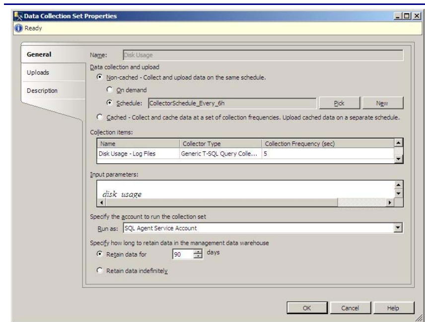
Figure 12. Disk Usage properties.
