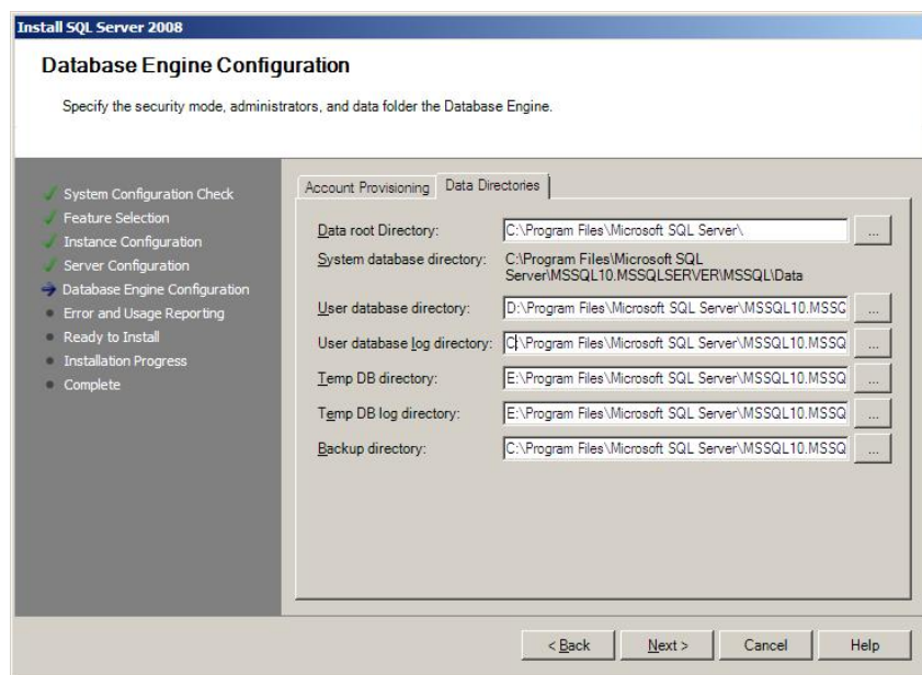
Figure 6. Setting file locations.
