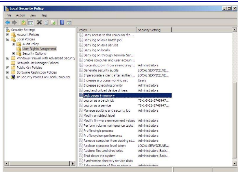
Figure 7. Selecting the Lock pages in memory setting.
